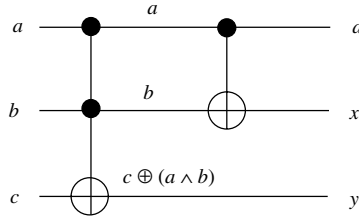
Figure 4.15 Binary addition circuit.
