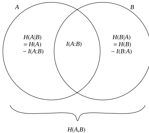
Figure 3.3 Relationships between the various entropies and the mutual information.
