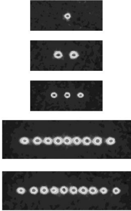
Figure 5.7 Ions in a string in a linear trap. (From Ref. [70]; with permission of Rainer Blatt.).
